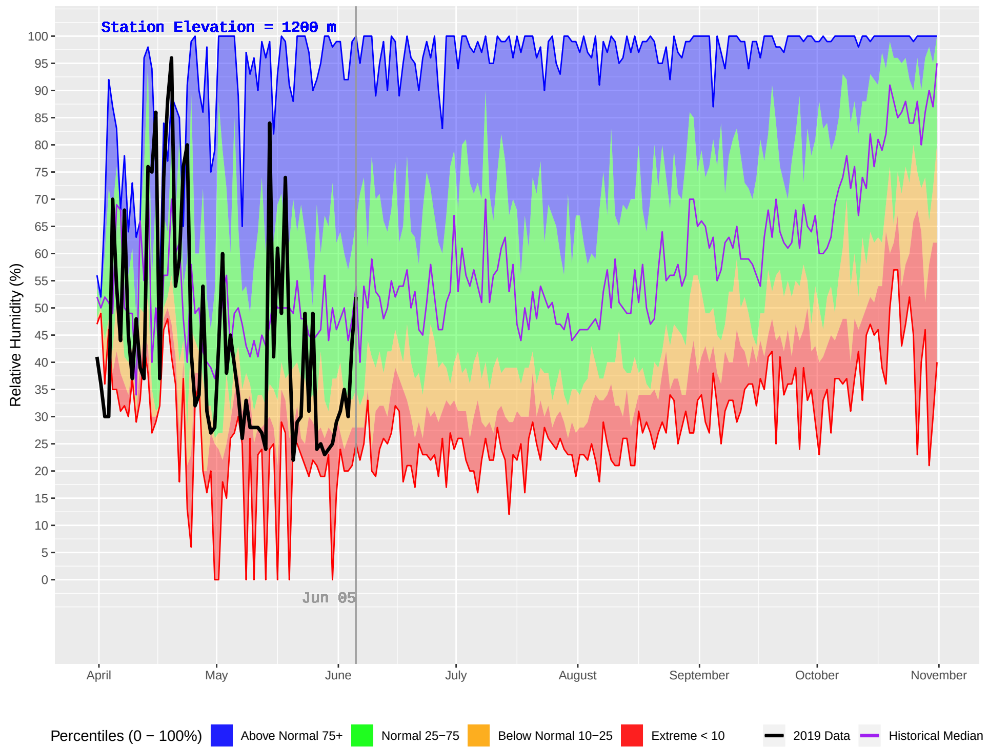
TSAR CREEK (361) : Historical (1986–2018) and Current (2019) Daily Relative Humidity
