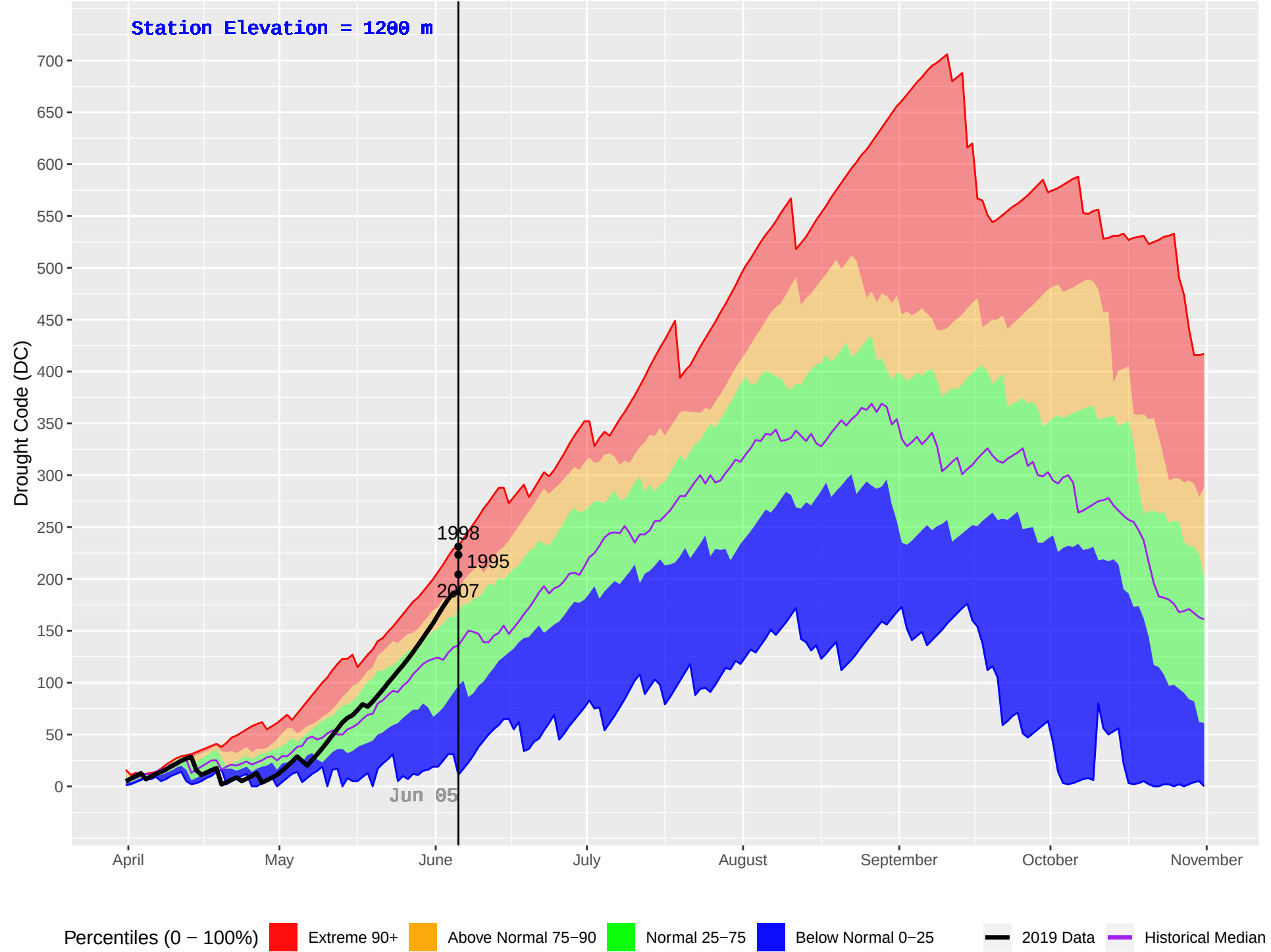
TSAR CREEK (361) : Historical (1986–2018) and Current (2019) Daily Drought Code (DC)
