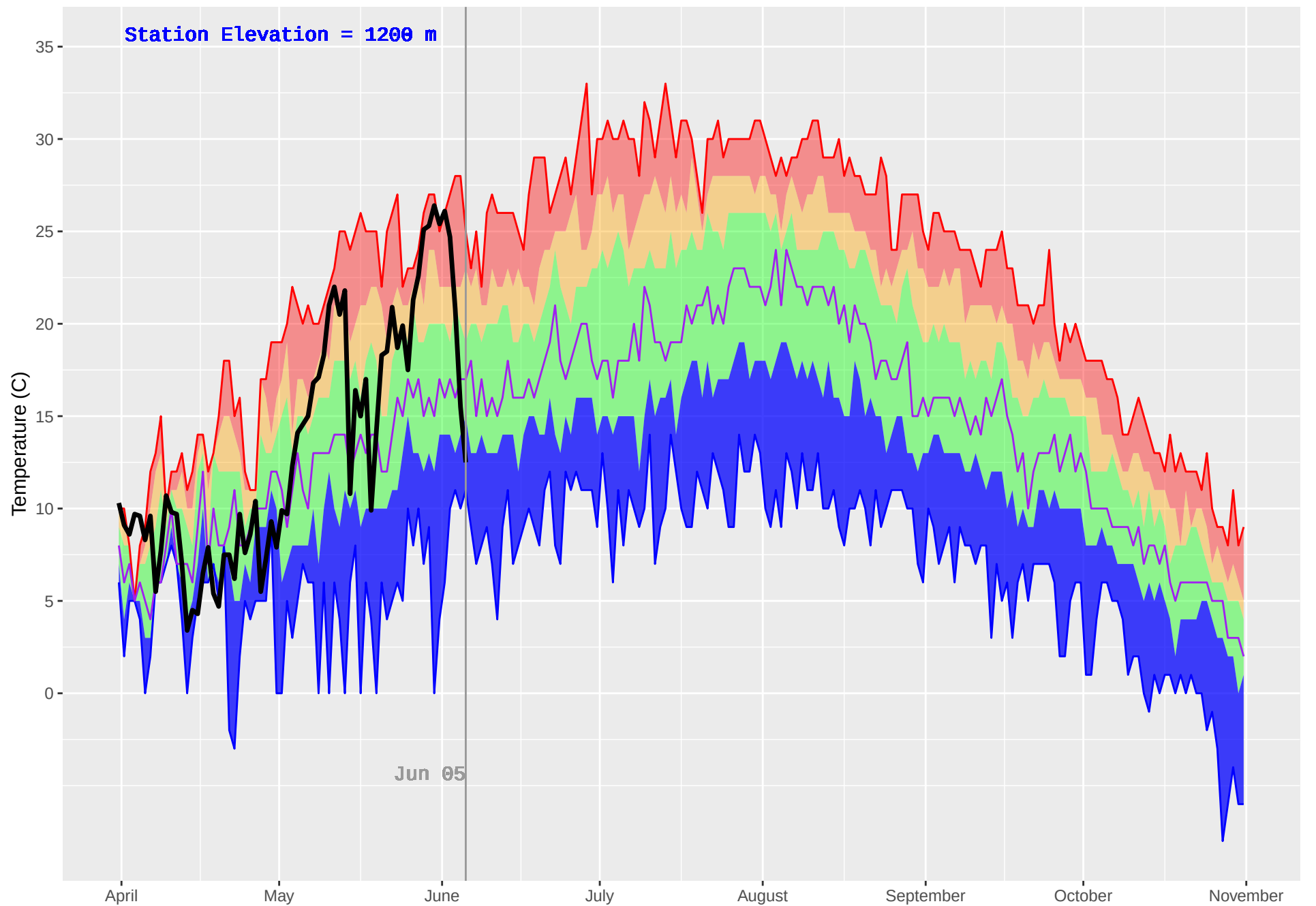
TSAR CREEK (361) : Historical (1986–2018) and Current (2019) Daily Temperature
