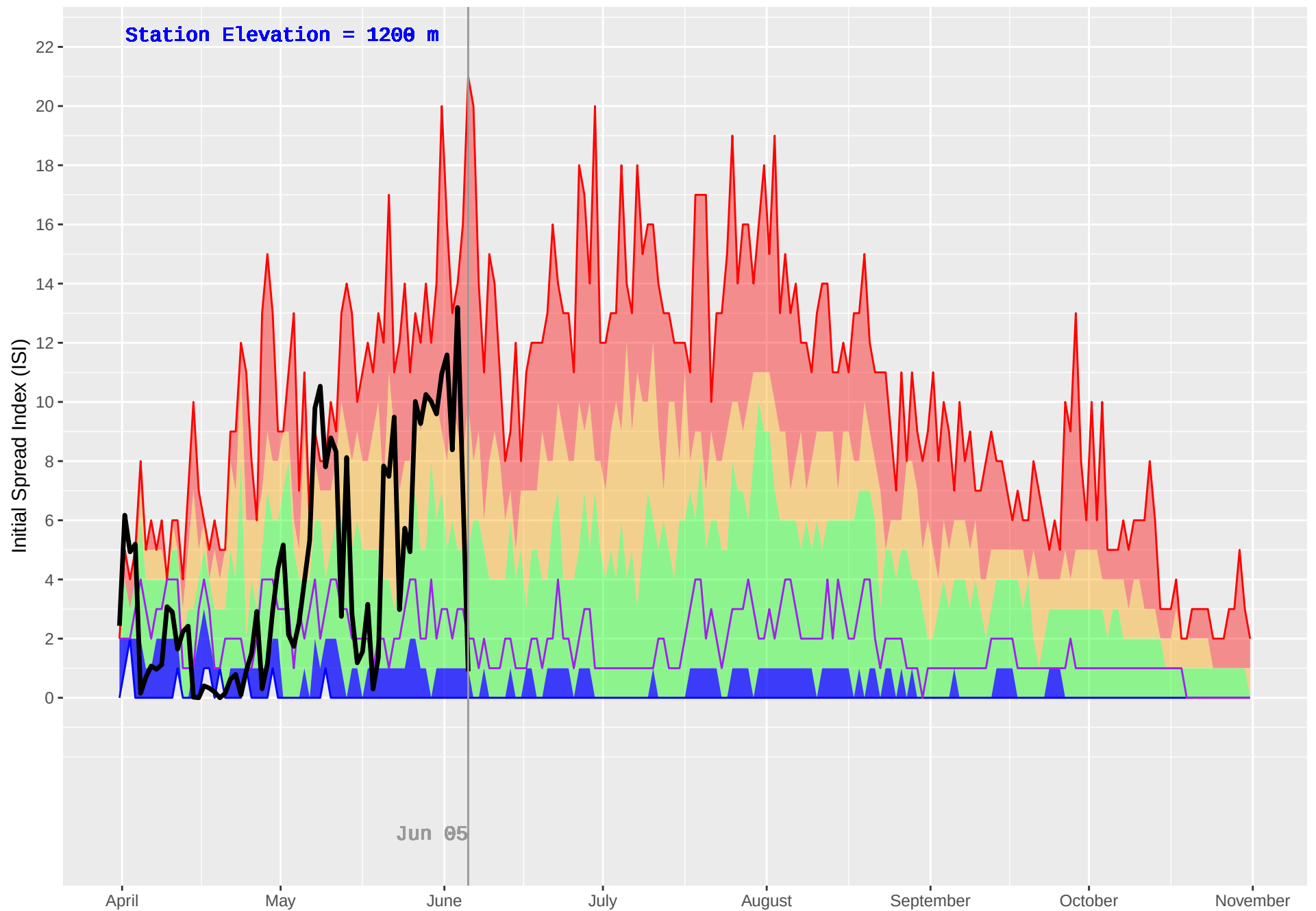
TSAR CREEK (361) : Historical (1986–2018) and Current (2019) Daily Initial Spread Index (ISI)
