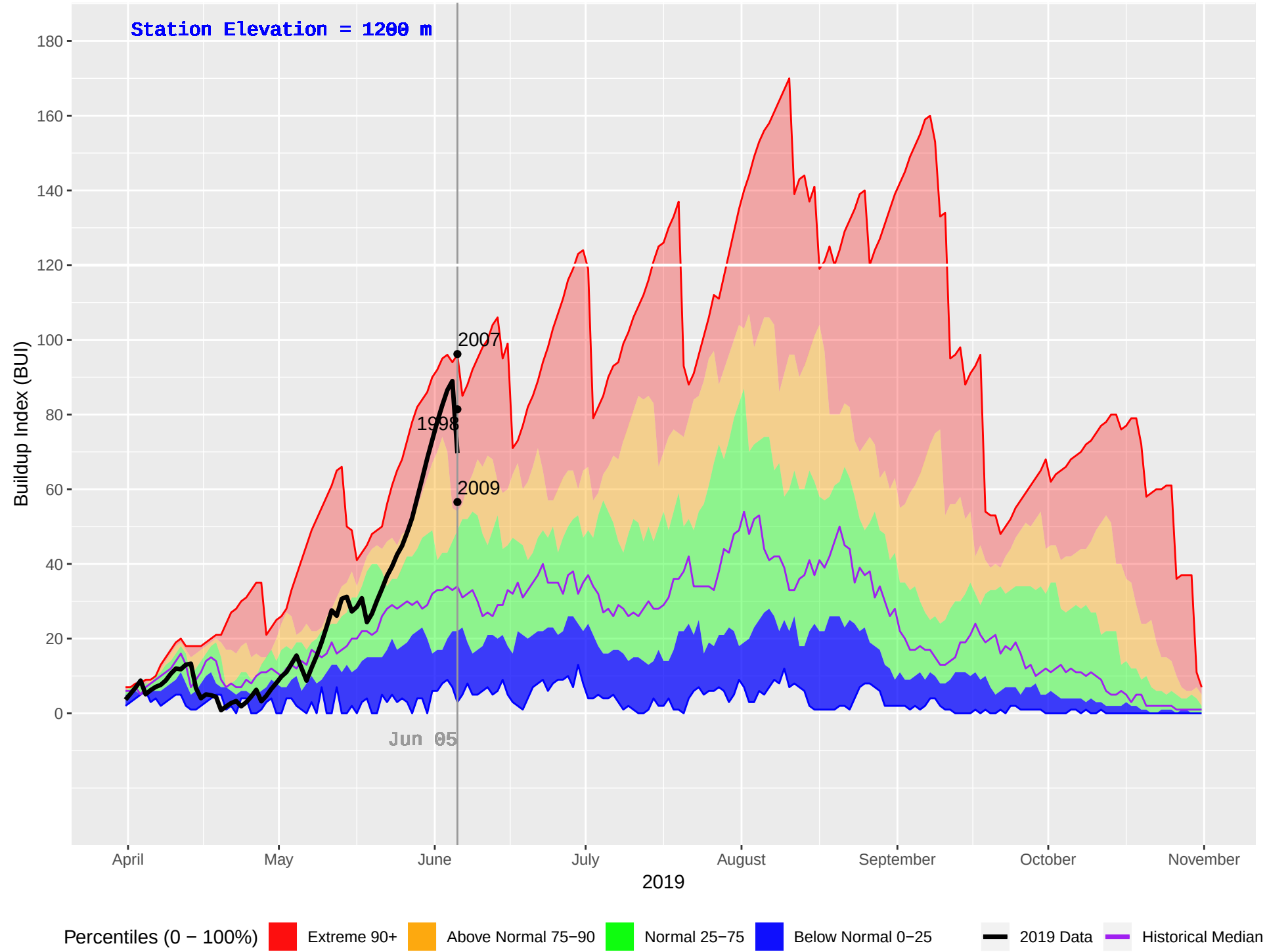
TSAR CREEK (361) : Historical (1986–2018), Current (2019) Daily Buildup Index (BUI)
