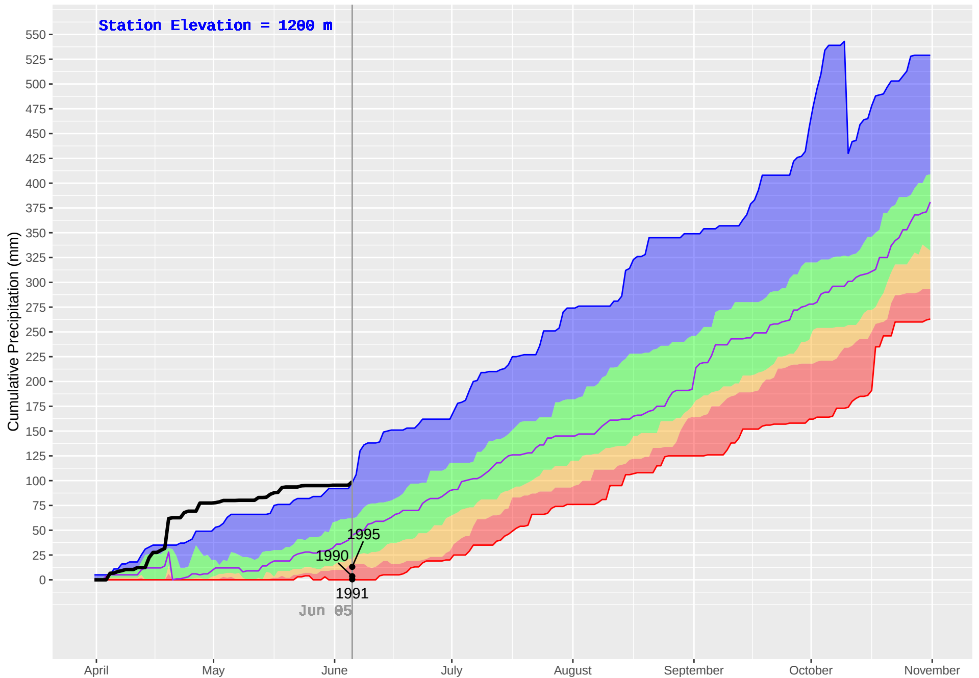
TSAR CREEK (361) : Historical (1986–2018), Current (2019) Daily Cumulative Precipitation
